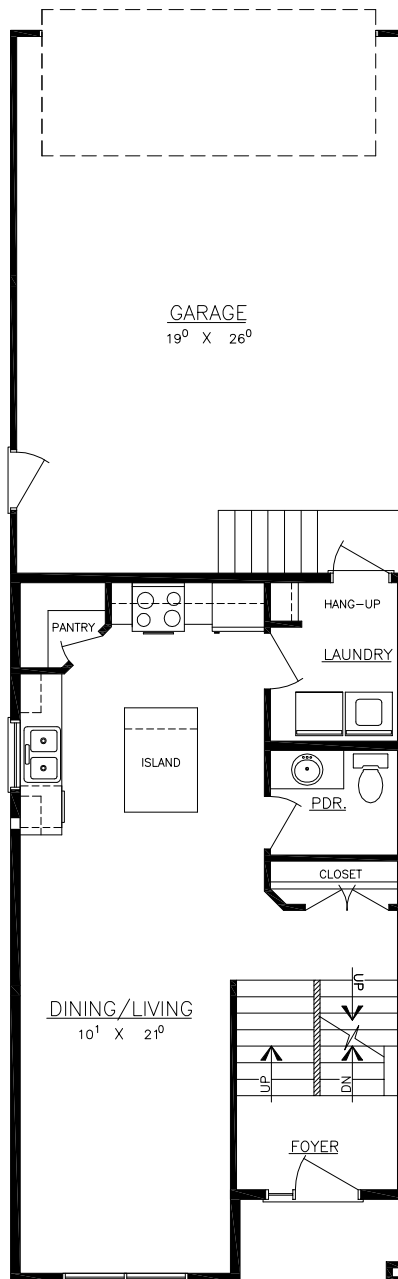
MAIN FLOOR AREA = 614 S.F.
